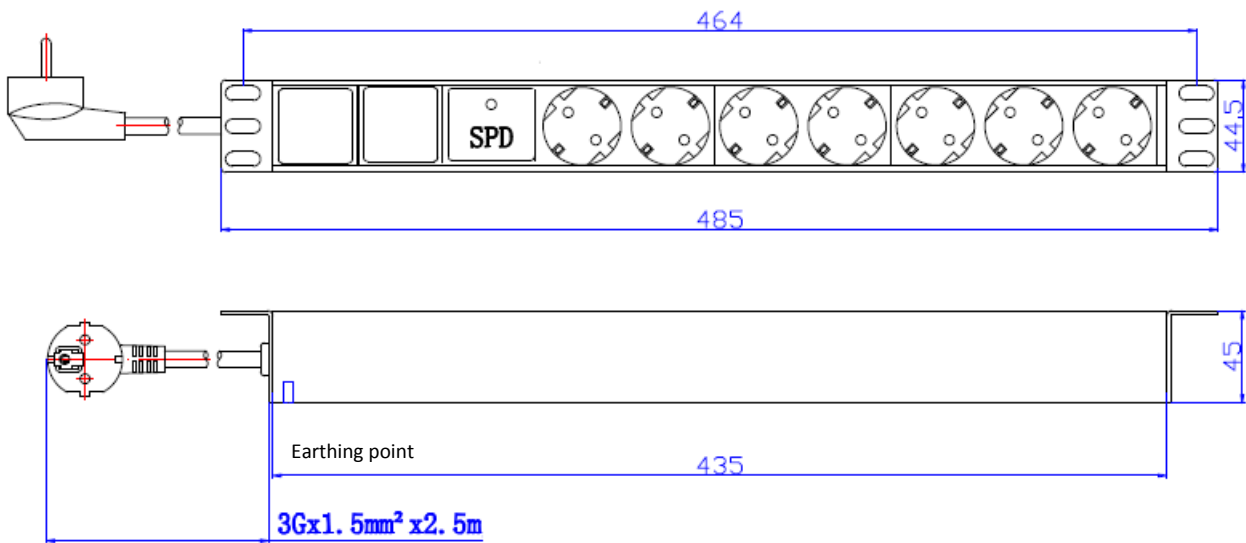
Connection diagram
